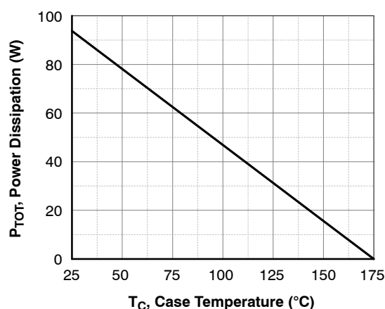
Figure 4. Power Derating
