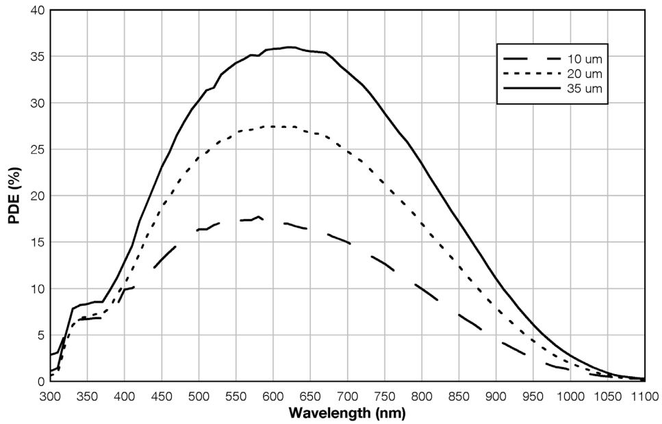
Figure 1. PDE vs. Wavelength
