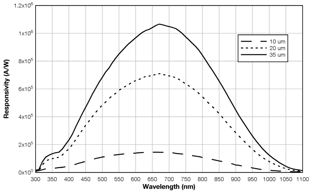
Figure 2. Responsivity vs. Wavelength
