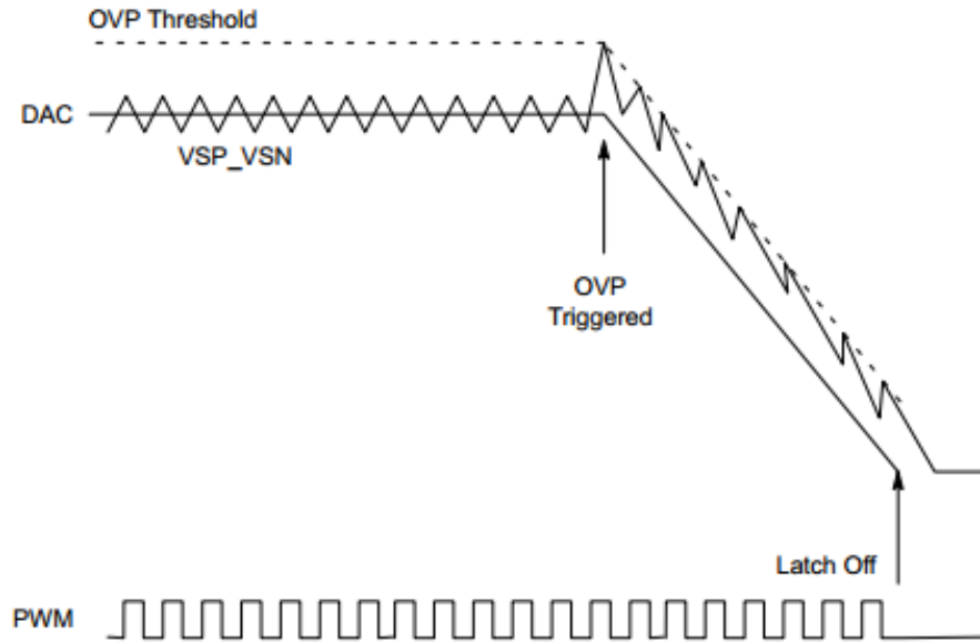
Figure 15. OVP during Normal Operation Mode
