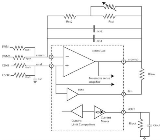
Figure 9. Total Current Sense Amplifier
