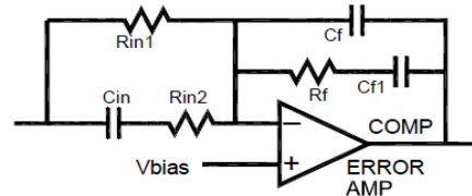
Figure 10. Error Amplifier
