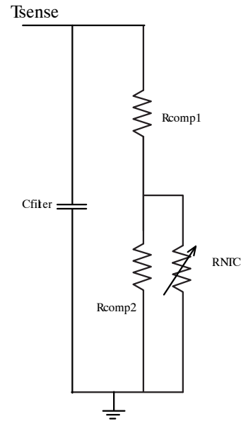
Figure 12. TSense Network
