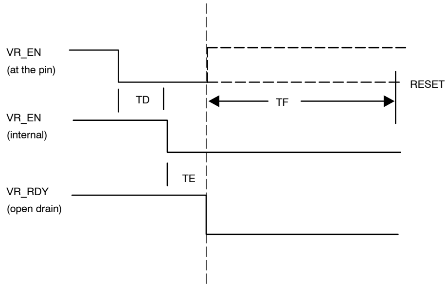
Figure 6. Shut-down Timing Diagram
