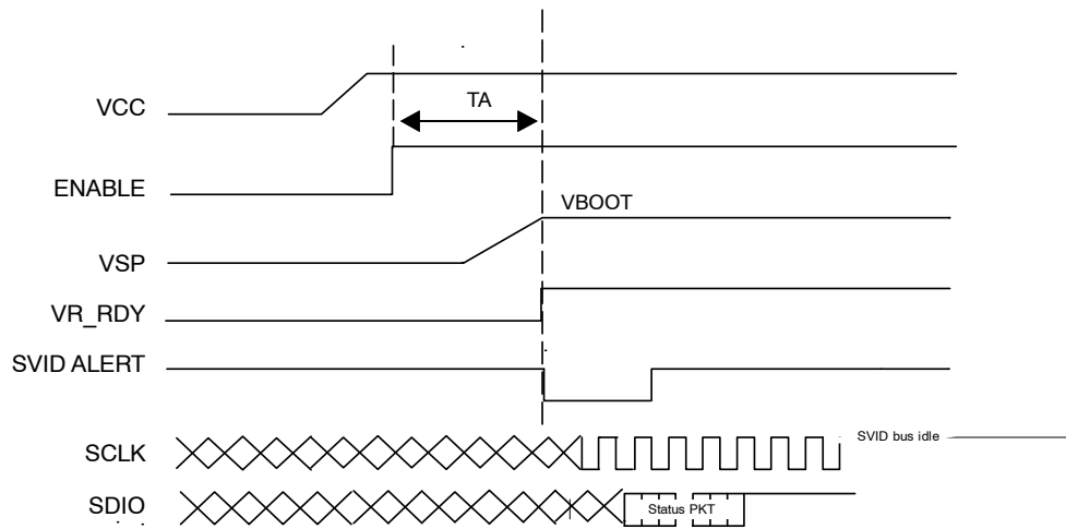
Figure 4. Start-up Timing Diagram – Non-zero VBOOT
