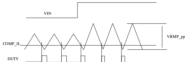
Figure 7. Ramp Feed-Forward
