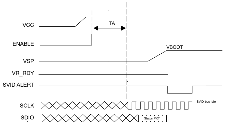
Figure 5. Start-up Timing Diagram – Zero VBOOT
