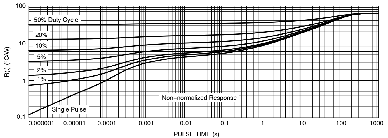
Figure 27. Duty Cycle for 1 \text{inch}^2 (645 \text{mm}^2 ) Spreader Board, DPAK 3-Lead
