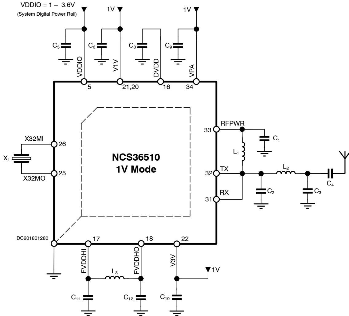
Figure 25. 1V System Application Diagram
