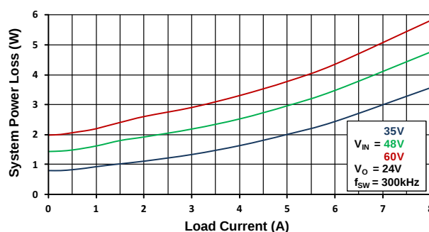
Figure 39. System Power Loss
