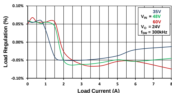
Figure 38. Load Regulation
