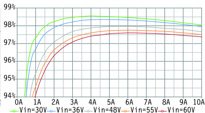
Figure 37. System Efficiency
