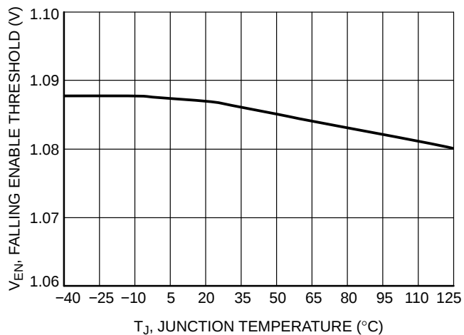
Figure 6. Falling Enable Threshold vs. Temperature
