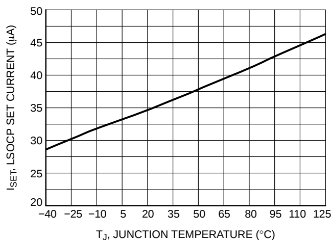
Figure 10. ISET Current vs. Temperature
