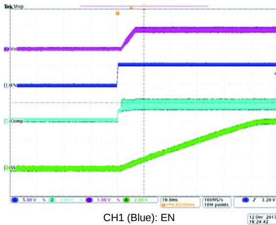
Figure 20. Typical Startup Waveforms ( V_{in} = 12\text{ V} , I_{out} = 25\text{ V} , V_{out} = 1\text{ V} )
