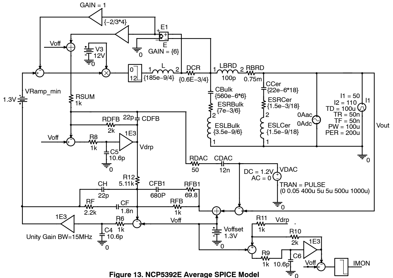
Figure 13. NCP5392E Average SPICE Model
