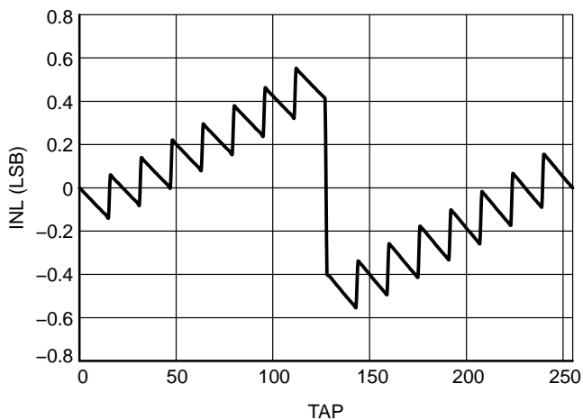
Figure 4. Average Integral Non-Linearity (V CC = 2.4 V) Resistor Mode
