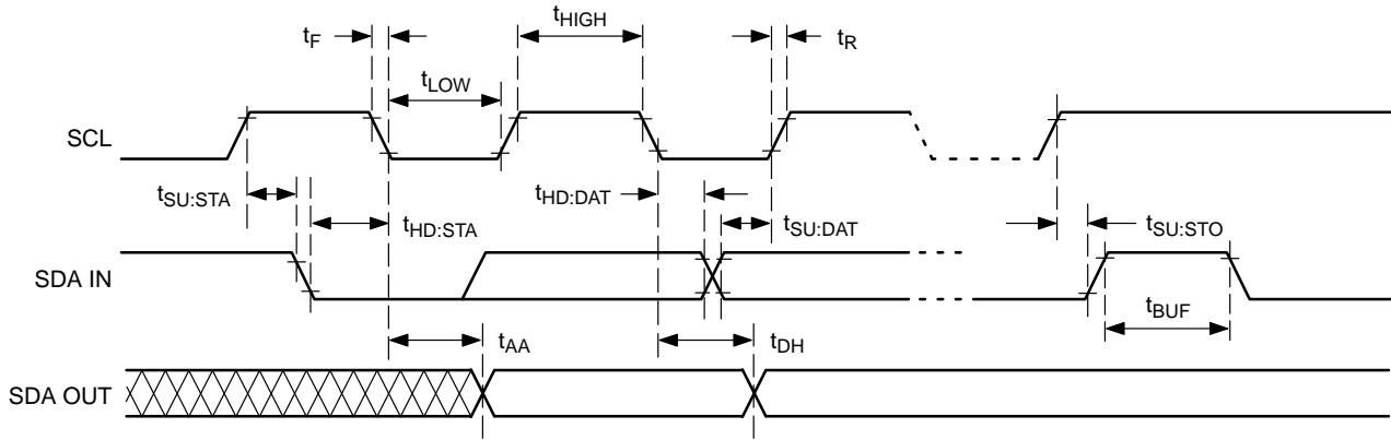
Figure 7. Bus Timing
