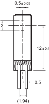
Cross section view A-A
