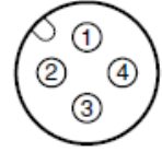
M12 Connector Pin Arrangement
