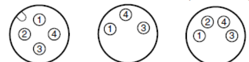
M12 Connector Pin Arrangement (See note 2.) M8 connector (3 pin) Pin Arrangement M8 Connector (4 pin) Pin Arrangement (See note 2.)
