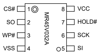
8-pin plastic SOP
