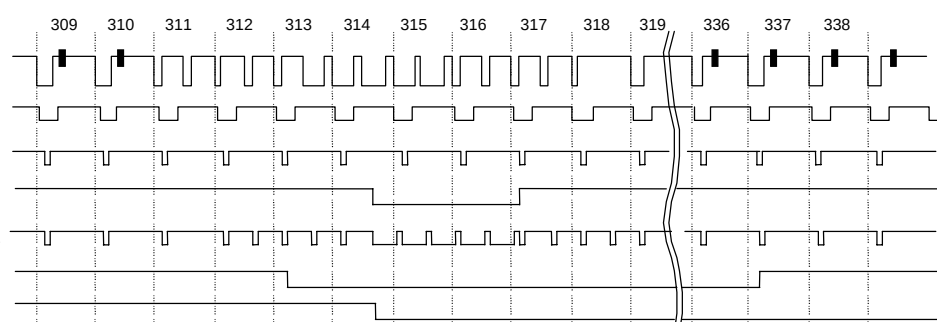
Vertical Sync Signals (50 Hz)
