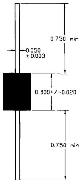
EPOXY CASE
