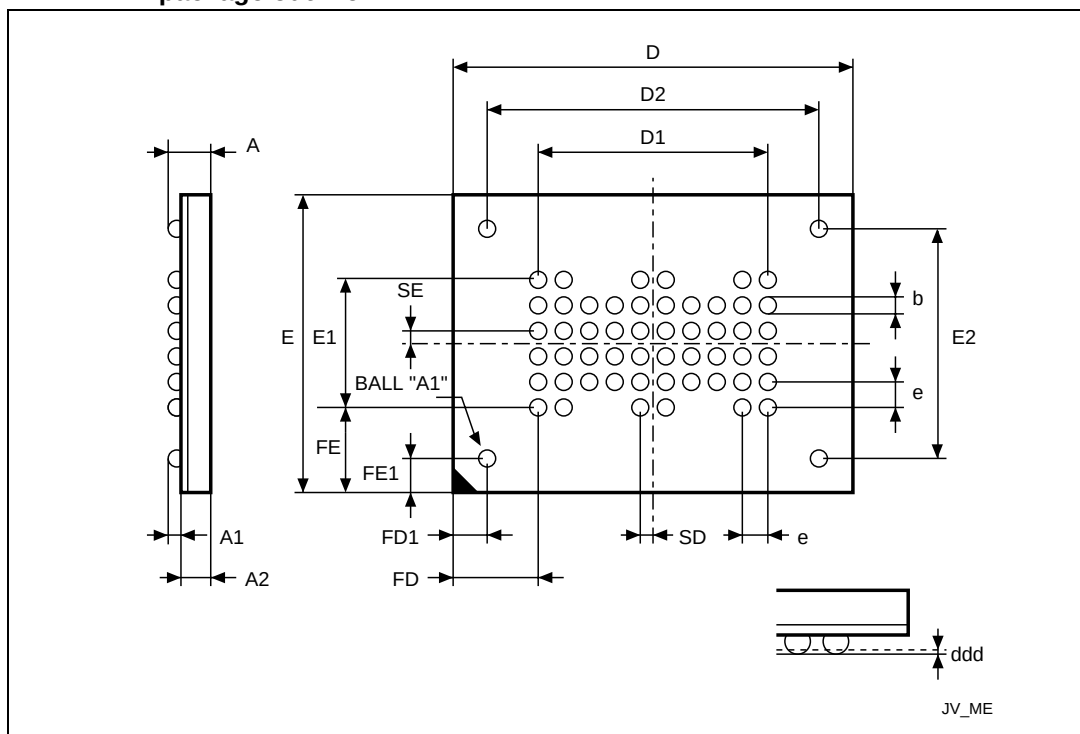
Figure 9. TFBGA56 8 \times 6 \times 1.2 mm, 10 \times 6 ball array - 0.5 mm pitch, bottom view package outline
