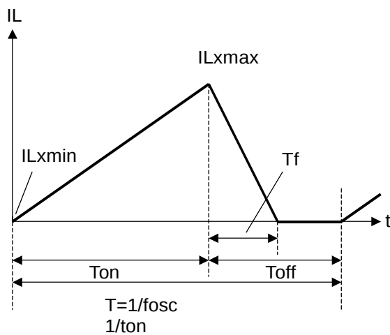
Discontinuous Mode
