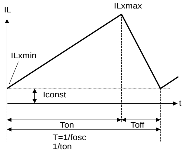
Continuous Mode
