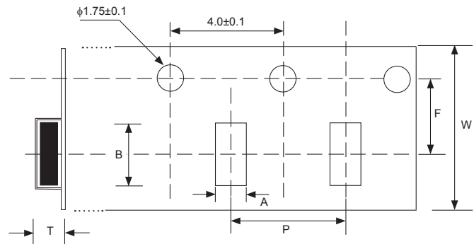
EMBOSSED PLASTIC CARRIER
