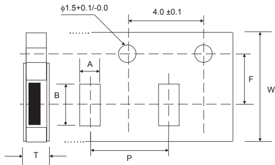
PAPER CARRIER
