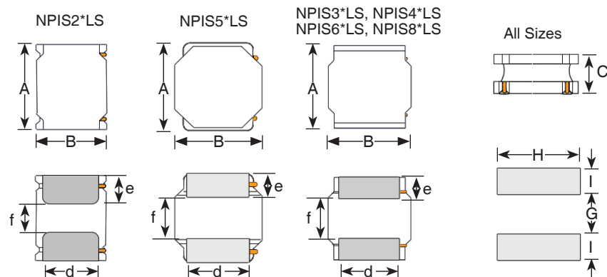
REFLOW SOLDERING LAND PATTERN (ALL SIZES)
