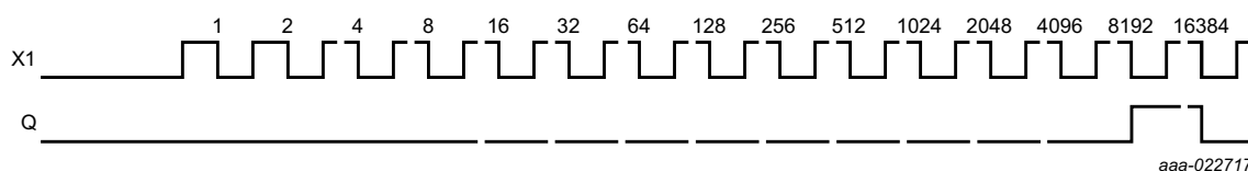
Fig 4. Timing diagram
