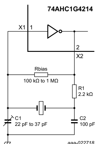
Fig 8. External component connection for a crystal oscillator
