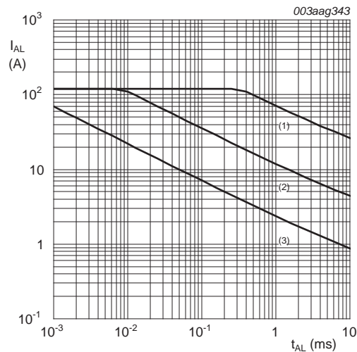
(1) T_{j(jst)} = 25^{\circ}C ; (2) T_{j(jst)} = 150^{\circ}C ; (3) Repetitive Avalanche
