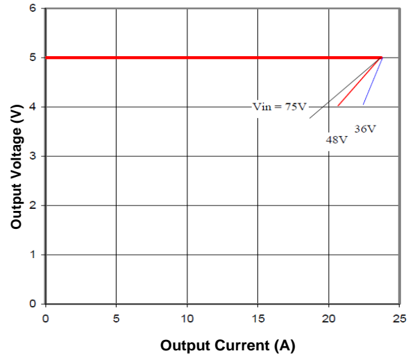
Figure 10. Output Characteristics
