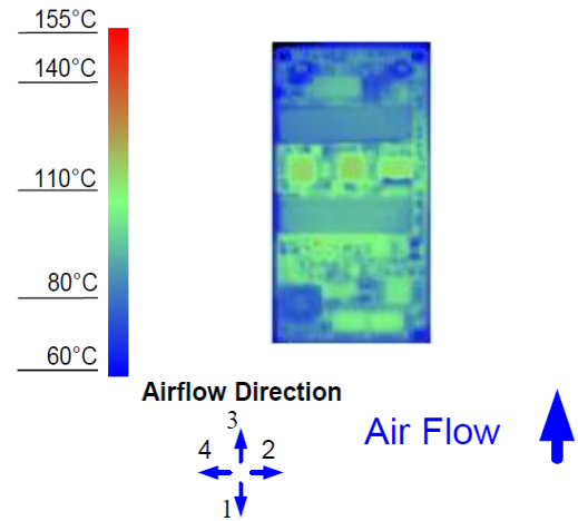
Figure 12. Thermal Image for Airflow Direction 2 (18.7A output, 55°C ambient, 200 LFM, typical V_{in} , open frame, socket interface)
