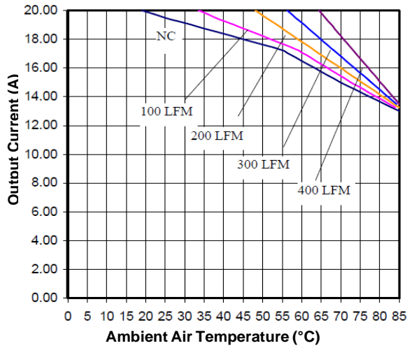
Figure 11. Current Derating Curve for Airflow Direction 2 (Ref. Figure 12 for Airflow Direction; V_{in} = 48V , open frame unit)
