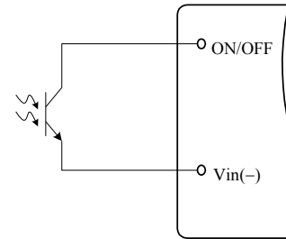
Figure 14. Opto Coupler Enable Circuit
