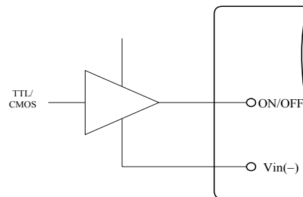
Figure 16. Direct Logic Drive
