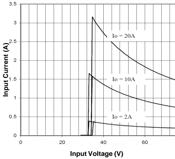
Figure 9. Input Characteristics
