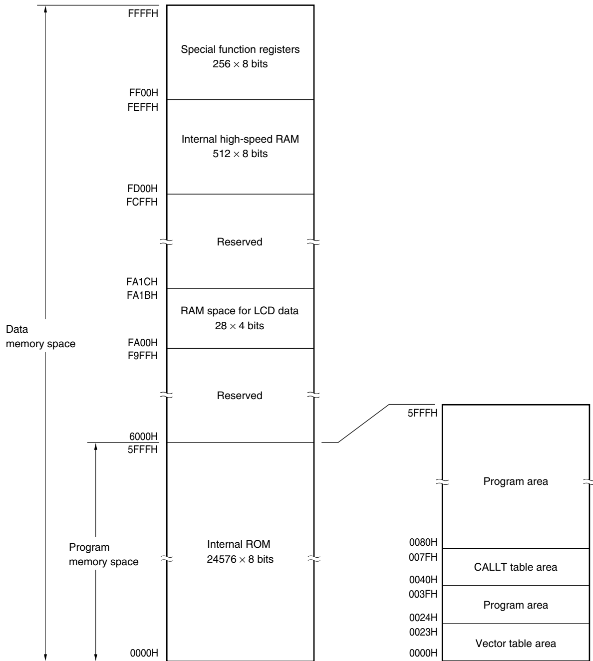
Figure 3-3. Memory Map ( \mu PD789407A and \mu PD789417A)
