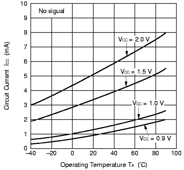
CIRCUIT CURRENT vs. OPERATING TEMPERATURE
