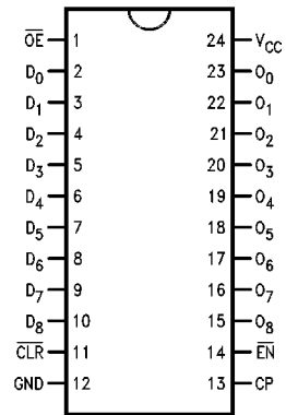
Pin Assignment for DIP and Cerpack
