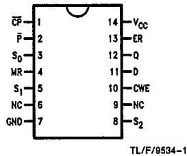
Pin Assignment for DIP, SOIC and Flatpak
