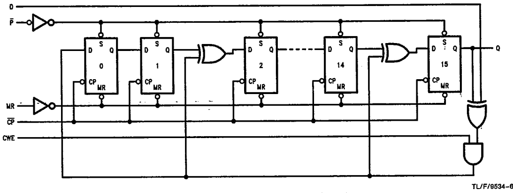
FIGURE 1. Equivalent Circuit for X^{16} + X^{15} + X^2 + 1
