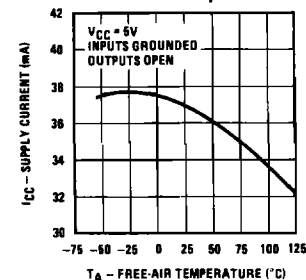
Supply Current (Both Drivers) vs Free-Air Temperature
