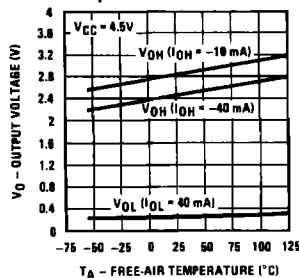
Output Voltage vs Free-Air Temperature
