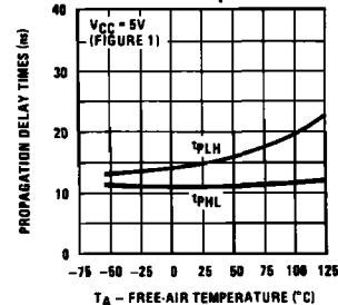
Propagation Delay Times vs Free-Air Temperature
