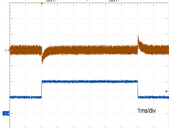
Transient Response ( V_{\text{IN}} = 48\text{V} , I_{\text{OUT}} = 0.5 to 1 to 0.5\text{A} , T_a = +25^{\circ}\text{C} ) Ch1 = V_{\text{OUT}} , 200mV/div, Ch2 = I_{\text{OUT}} , 500mA/div
