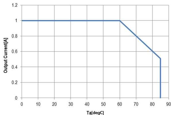
Thermal Derating Unit under test (UUT) is covered by acrylic box to avoid airflow. ( V_{\text{IN}} = 48\text{V} , See Technical Notes)
