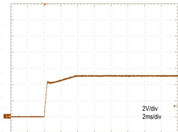
V_{\text{OUT}} Start-up ( V_{\text{IN}} = 48\text{V} , I_{\text{OUT}} = 2\text{A} , T_a = +25^{\circ}\text{C} )
