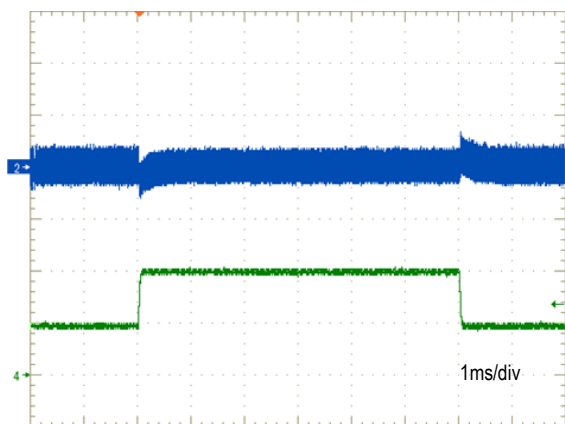
Transient Response ( V_{\text{IN}} = 48\text{V} , I_{\text{OUT}} = 1 to 2\text{A} , T_a = +25^{\circ}\text{C} ) Ch2 = V_{\text{OUT}} , 200mV/div, Ch4 = I_{\text{OUT}} , 1A/div
