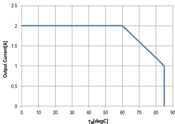
Thermal Derating Unit under test (UUT) is covered by acrylic box to avoid airflow. ( V_{\text{IN}} = 48\text{V} , See Technical Notes)
