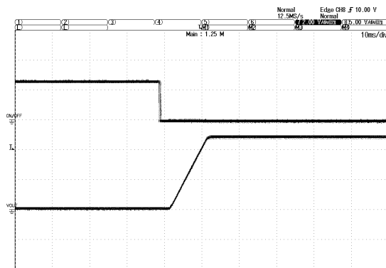
Enable Turn On – Negative Logic (Vin = 54V, Iout = 67A)
