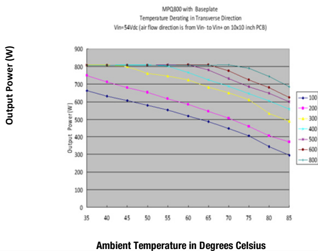
Output Power Derating Baseplate (Vin=54V)
