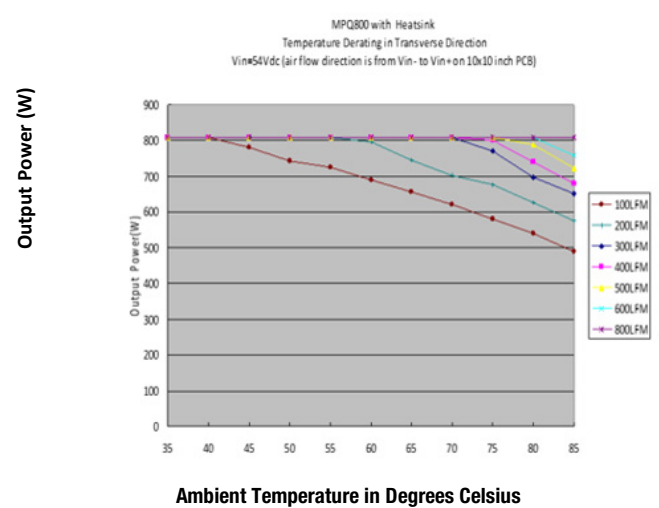
Output Power Derating 0.5" Heatsink (Vin=54V)
