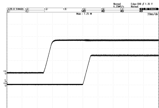
Vin Turn On (Vin = 54V, Iout = 67A)
