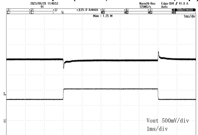
Transient Response (Vin = 54V, 50%-75%-50% Load, 1A/μs)
