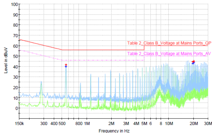
Conducted emissions performance, Negative Line CISPR 32, Class B, full load
