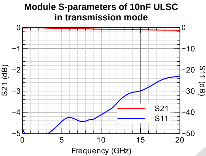
Figure 2 - 10nF ULSC measurement results (module of S-parameters)
