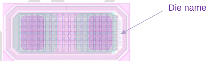
Figure 8 – Layout view
