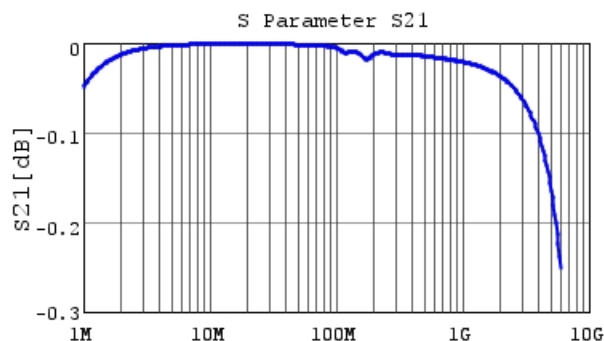
GRM1887U1A153JA01 S21 DCOV, 25degC
