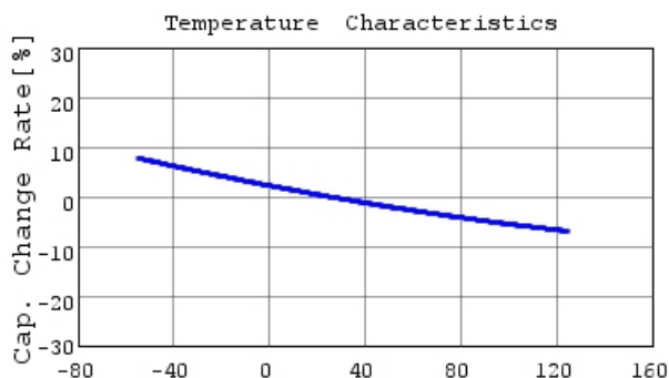
GRM1887U1A153JA01 C-Temp. capchange, DCOV, 1
