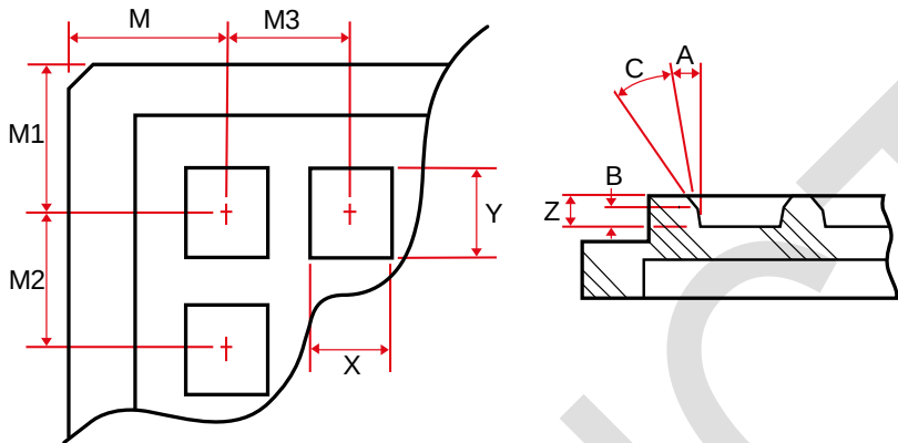
Figure 15 - Waffle pack drawing
