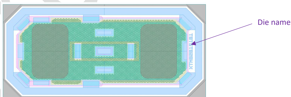
Figure 8 – Layout view
