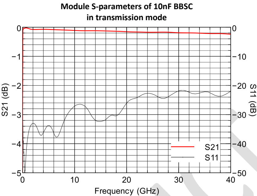
Figure 2 - 10nF BBSC measured results (module of S-parameters)
