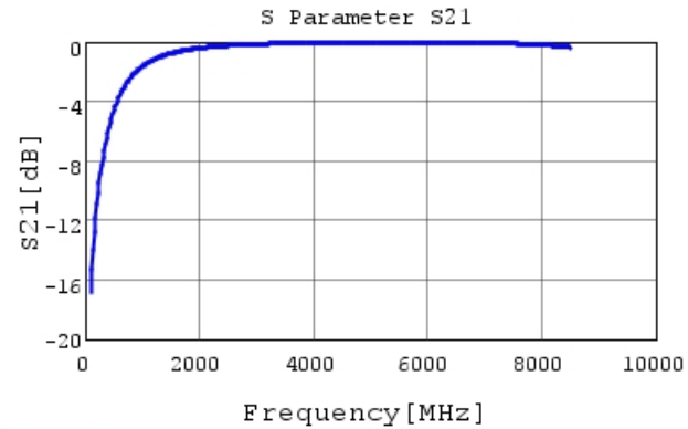
GJM1555C1H2R3BB01 S21 DCOV, 25degC
