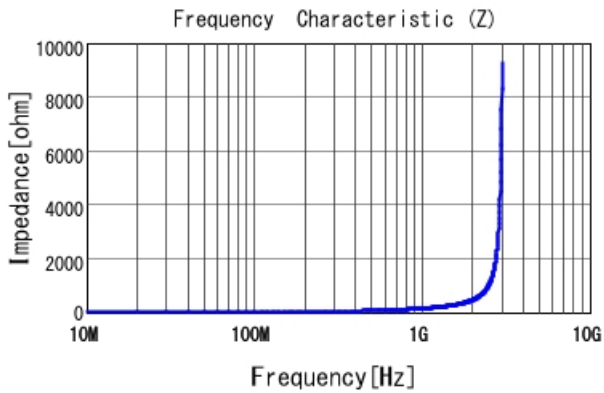
■ LQP03TN22NH02 |Z|
