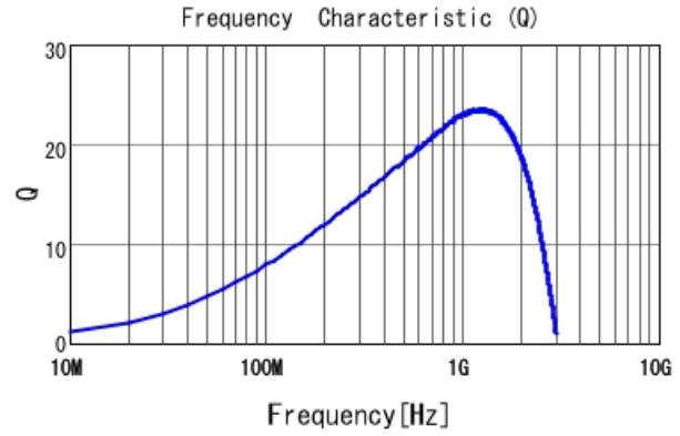
■ LQP03TN22NH02 Q
