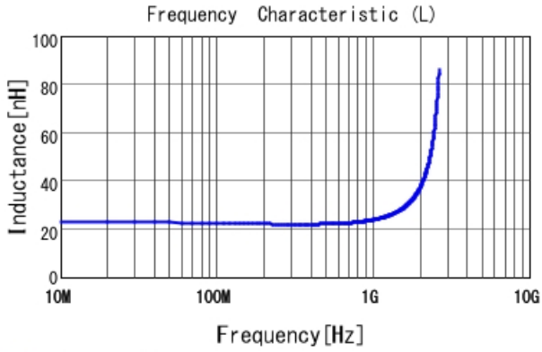
■ LQP03TN22NH02 L
