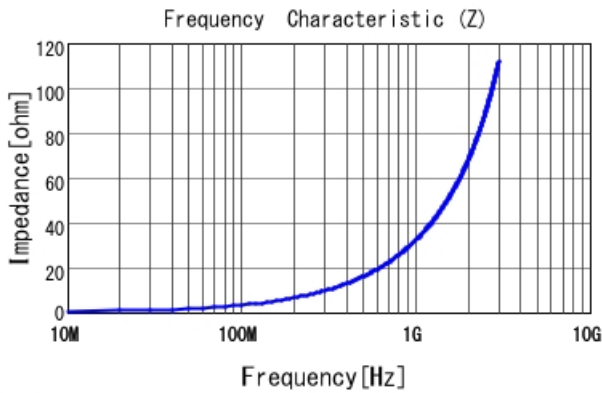
■ LQP15MN5N1B02 |Z|
