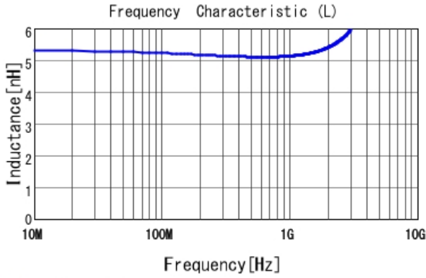
■ LQP15MN5N1B02 L
