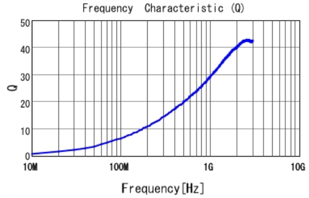
■ LQP15MN5N1B02 Q
