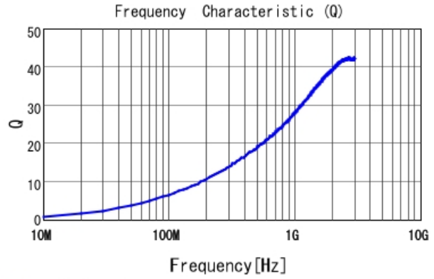
■ LQP15MN4N3B02 Q
