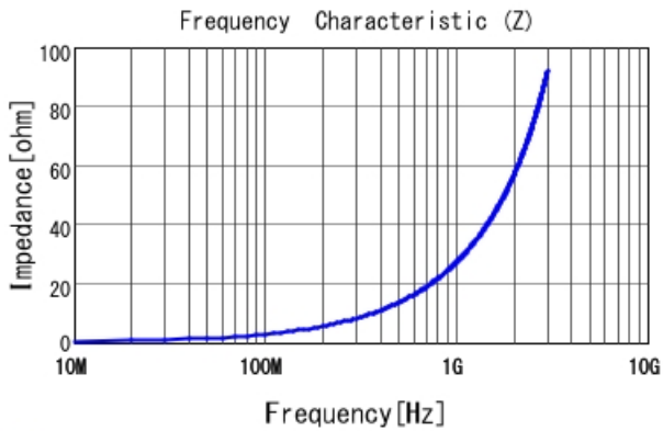
■ LQP15MN4N3B02 |Z|
