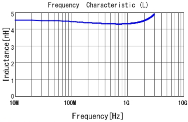
■ LQP15MN4N3B02 L
