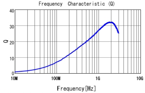
■ LQP15MN12NG02 Q
