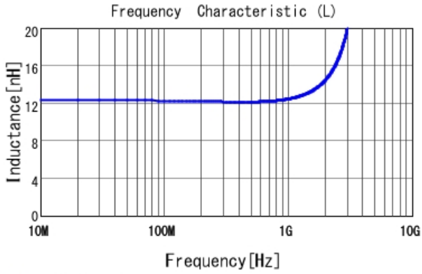
■ LQP15MN12NG02 L
