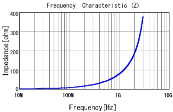
■ LQP15MN12NG02 |Z|
