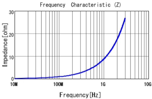
■ LQP15MN1N4W02 |Z|
