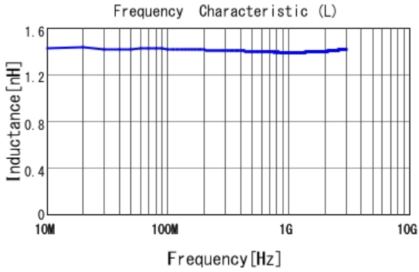
■ LQP15MN1N4W02 L
