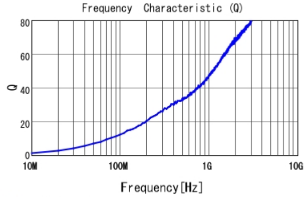
■ LQP15MN1N4W02 Q
