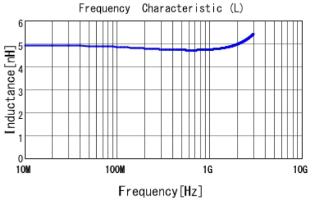
■ LQP15MN4N7B02 L
