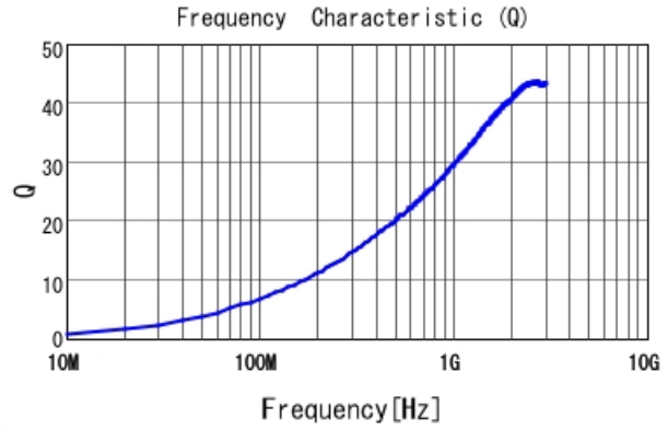
■ LQP15MN4N7B02 Q
