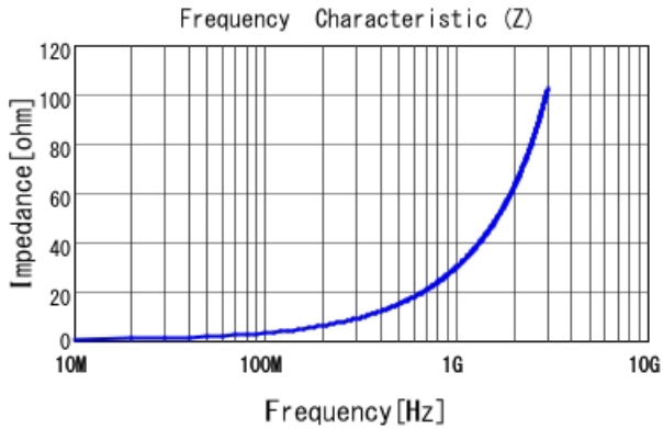
■ LQP15MN4N7B02 |Z|
