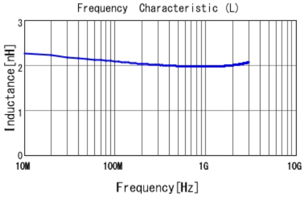
■ LQP03TN2N0B02 L
