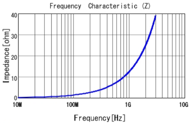
■ LQP03TN2N0B02 |Z|
