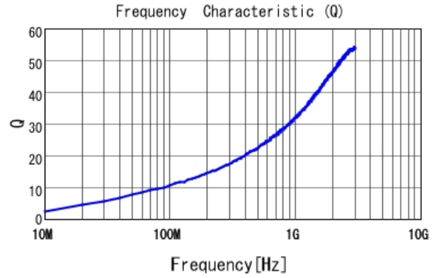
■ LQP03TN2N0B02 Q
