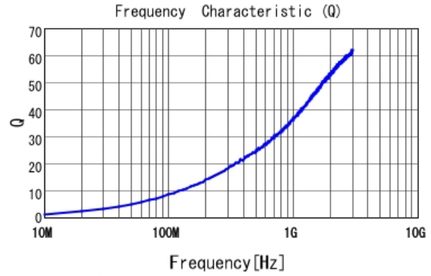
■ LQP15MN2N0B02 Q
