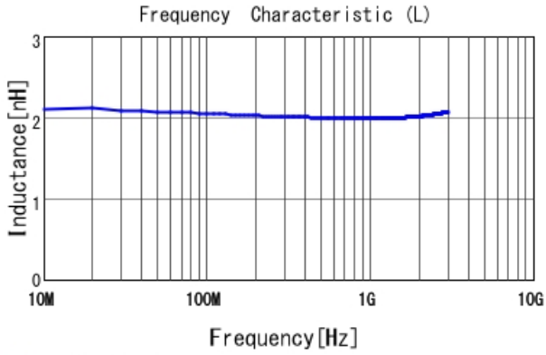
■ LQP15MN2N0B02 L
