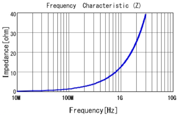
■ LQP15MN2N0B02 |Z|
