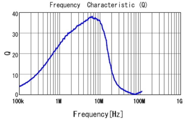
■ LQM21PN2R2MC0 Q
