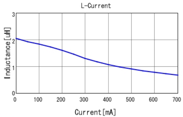
■ LQM21PN2R2MC0 L-Current 20degC
