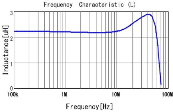
■ LQM21PN2R2MC0 L
