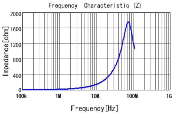
■ LQM21PN2R2MC0 |Z|
