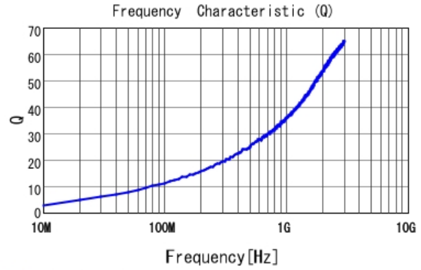
■ LQP03TN1N2B02 Q
