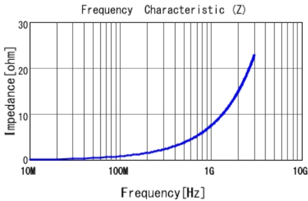
■ LQP03TN1N2B02 |Z|
