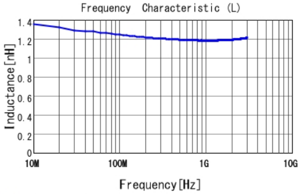
■ LQP03TN1N2B02 L
