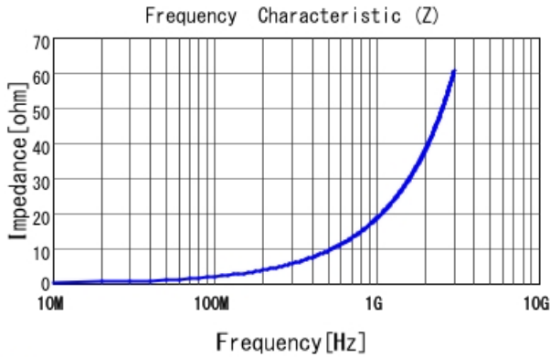
■ LQP03TN3N0B02 |Z|
