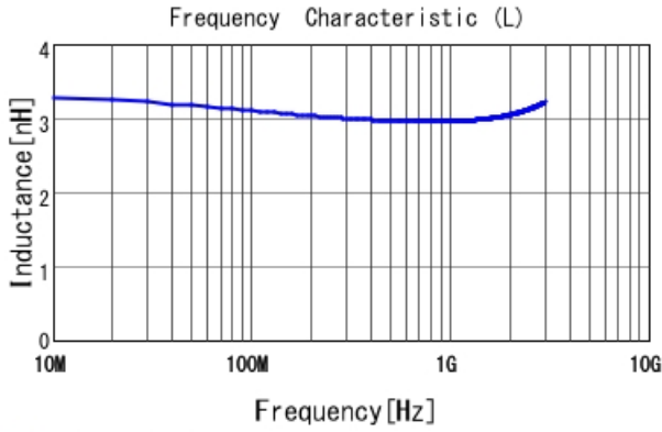
■ LQP03TN3N0B02 L
