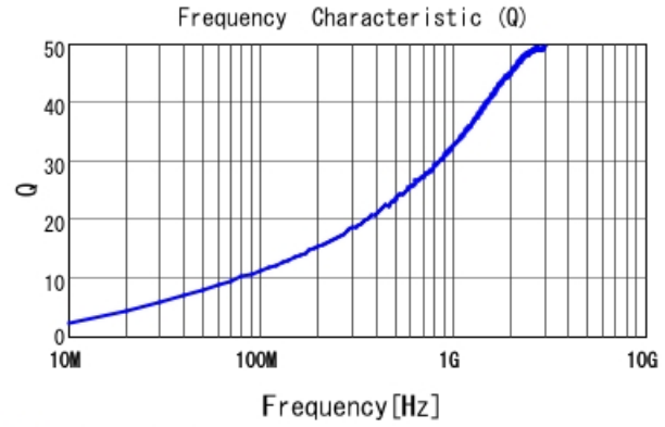
■ LQP03TN3N0B02 Q
