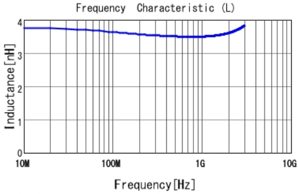
■ LQP15MN3N5W02 L
