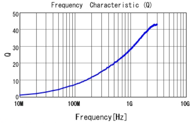
■ LQP15MN3N5W02 Q
