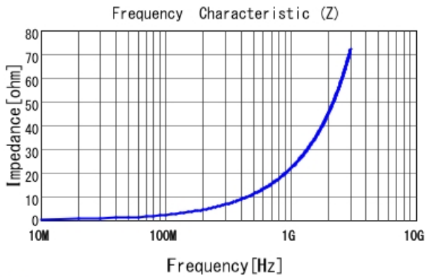
■ LQP15MN3N5W02 |Z|
