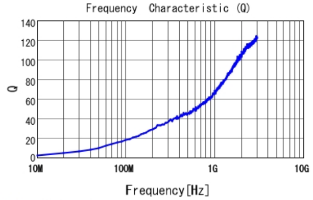
■ LQP15MN1N2W02 Q
