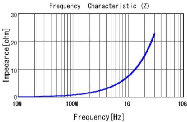
■ LQP15MN1N2W02 |Z|
