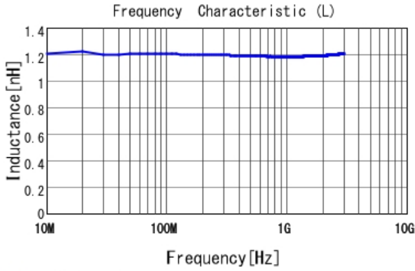
■ LQP15MN1N2W02 L
