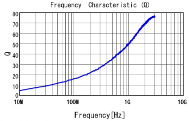
■ LQG15HN2N0S02 Q
