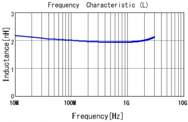
■ LQG15HN2N0S02 L
