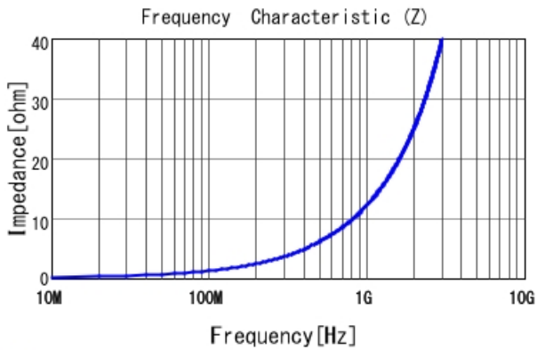
■ LQG15HN2N0S02 |Z|
