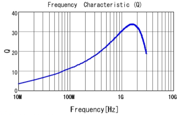
■ LQG15HN9N1J02 Q
