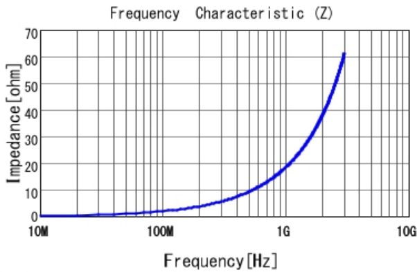
■ LQG15HN3N0S02 |Z|
