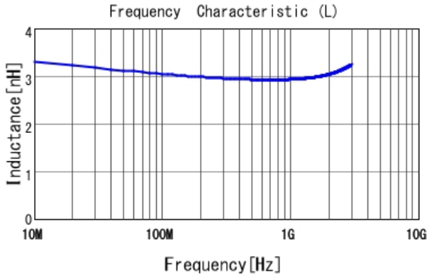
■ LQG15HN3N0S02 L
