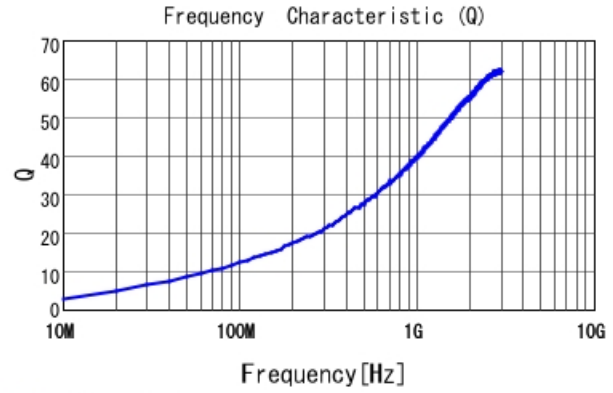
■ LQG15HN3N0S02 Q
