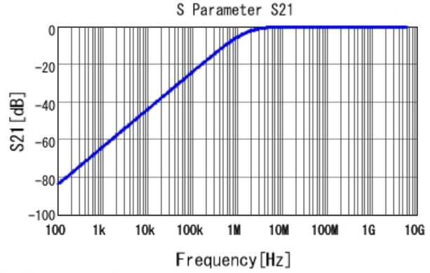
■ GCM155R71H102KA37 S21 DCOV, 25degC
